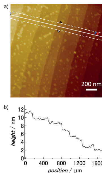
Figure 3. a) AFM image of the (010) surface of PESD-1 ⊃Guest. b) Averaged topographic profile of the portion of the surface enclosed within the dotted lines in (a). The AFM topographic image of the (010) surface exhibits terrace structures with widths in the range of 100–400 nm. The stepped structure displays discrete displacements of approximately 1.5 nm per step, which corresponds to the length of the b axis (1.41 nm), and reveals the flat nature of the (010) surface at the nanoscale (as observed previously for other PCPs/MOFs [17] ).
